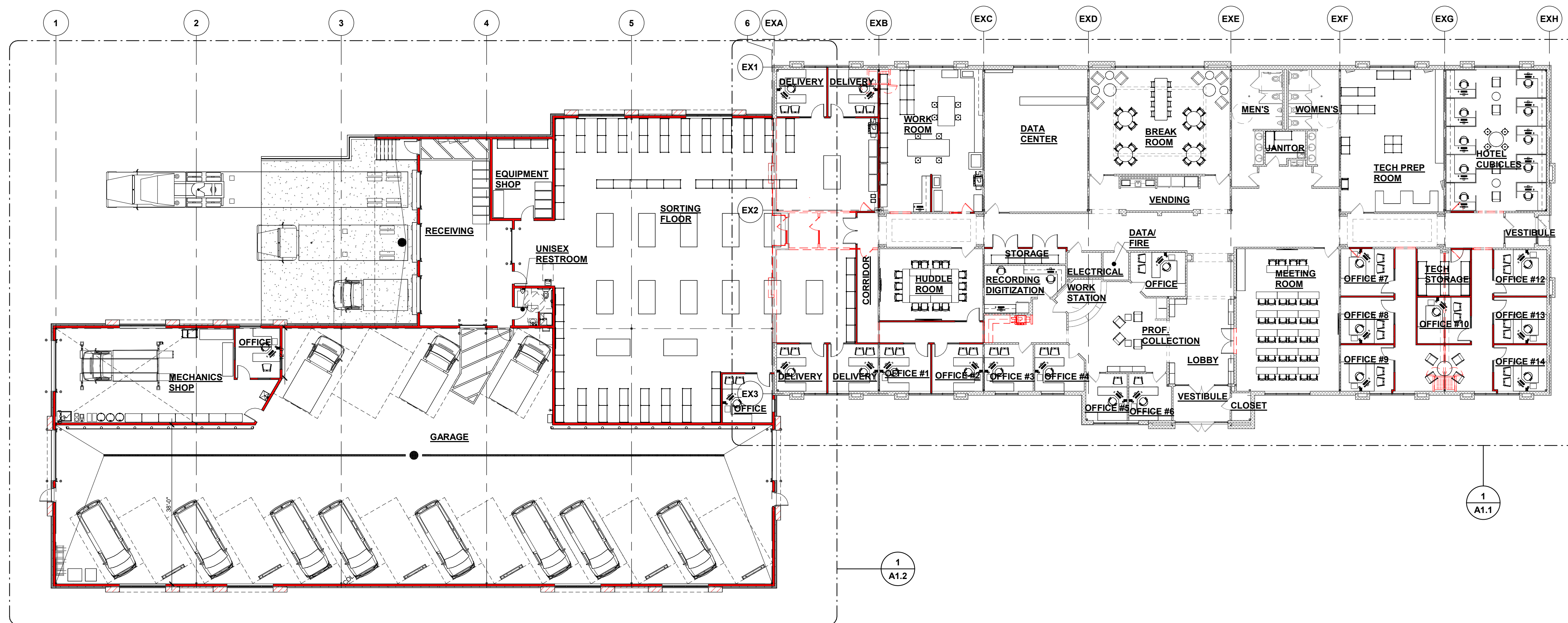
NORTH OVERALL FLOOR PLAN 1/16" = 1'-0"
